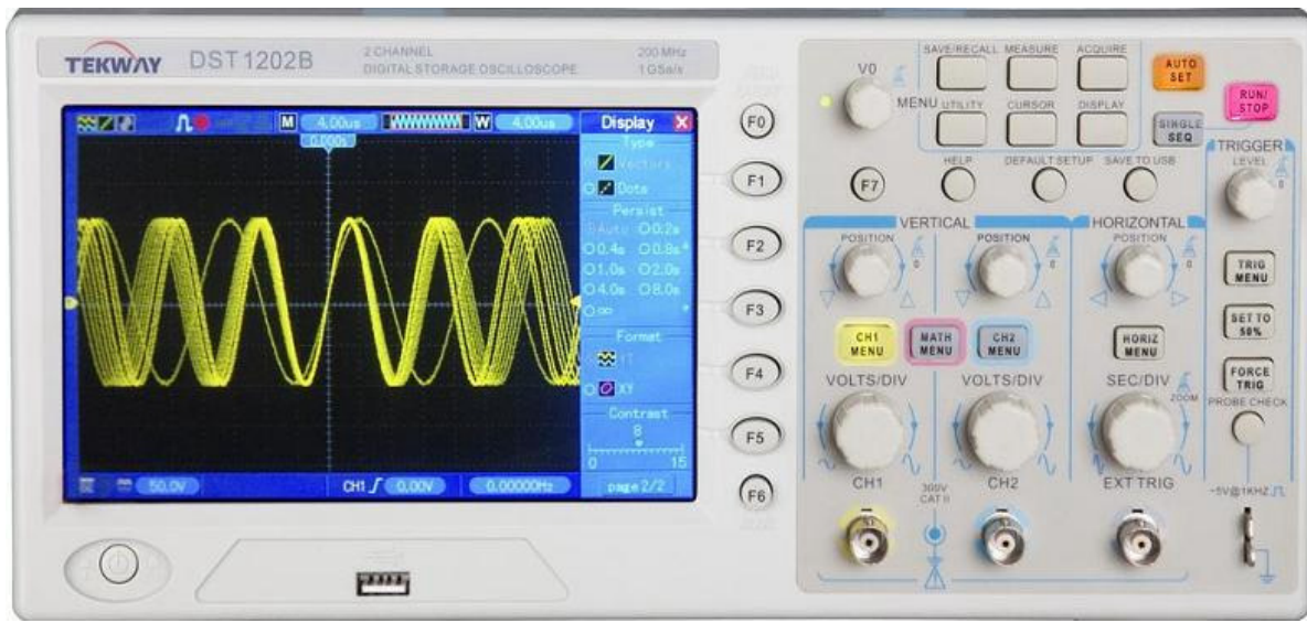
Front Panel of DST B Series
